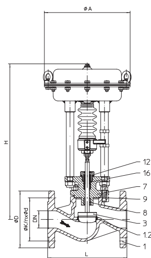
Fig. 440 Packing ring
